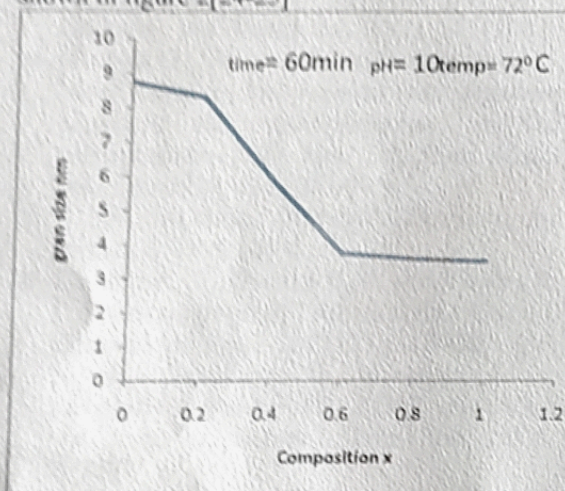
Figure 3: Graph between the composition parameters with grain size.
