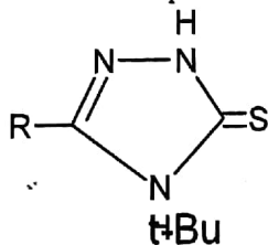
4-tert-butyl-5-aryl-2,4-dihydro-3H 1,2,4-triazole-3-Thione
