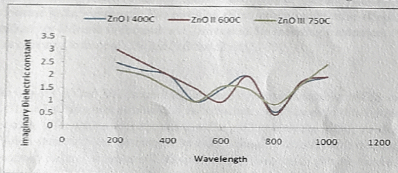
Figure 8: Variation of the imaginary dielectric constant as a function of wavelength for ZnO thin film.
