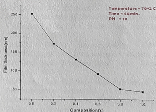
Figure 2: Graph between the composition parameter (x) with film thickness.
