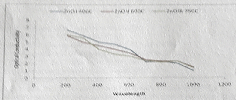
Figure 10: Variation of the optical conductivity as a function of wavelength for ZnO thin films
