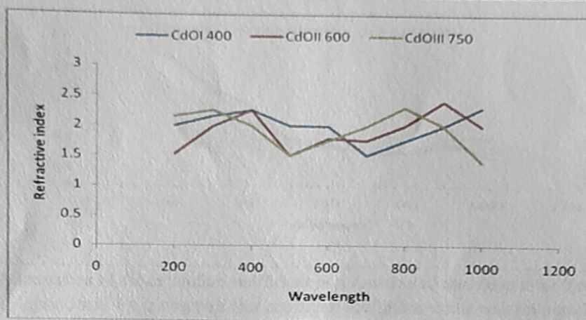
Figure1: Variation of the refractive index as a function of wavelength for CdO thin film.
